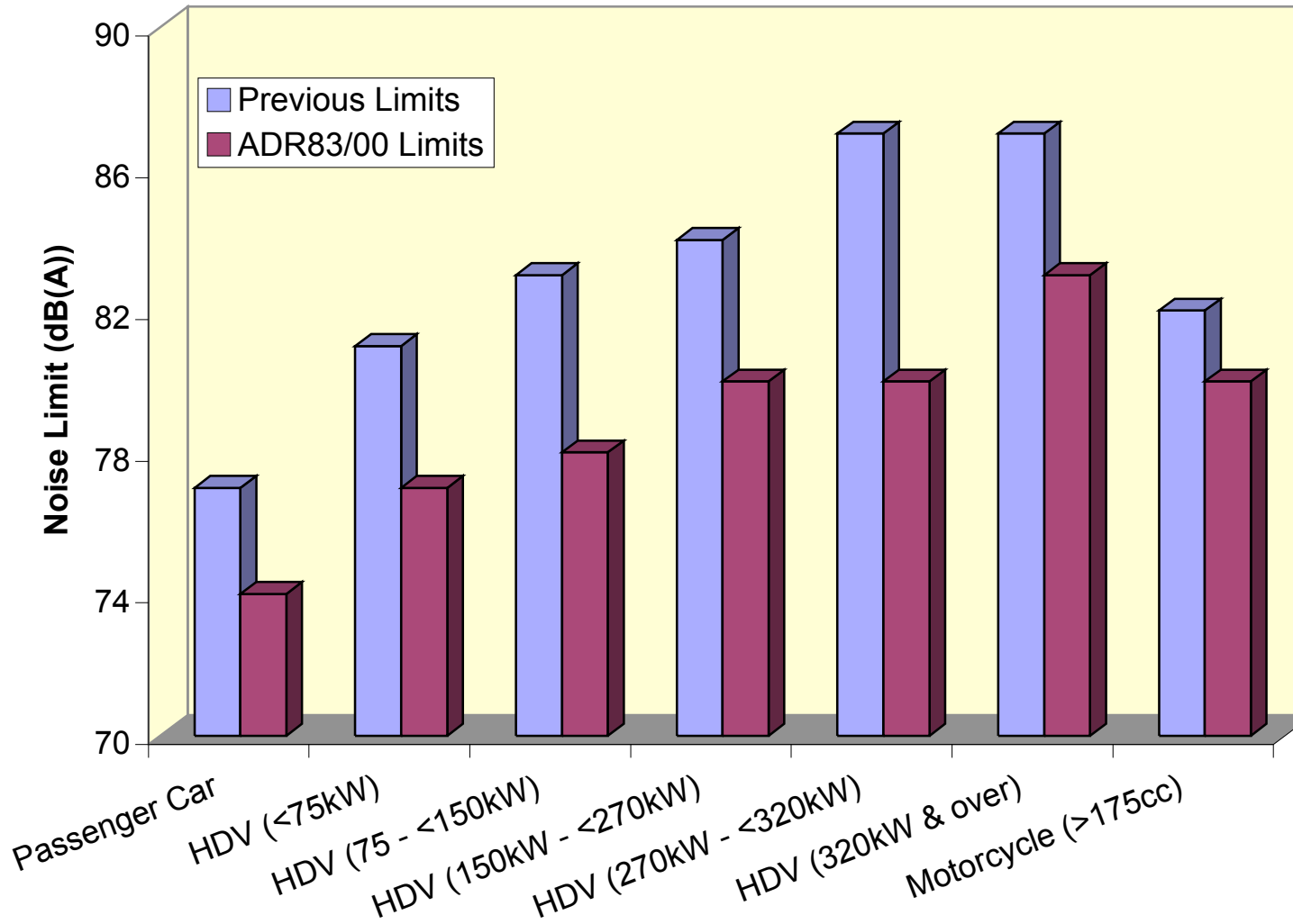
Comparison of Vehicle Noise Limits under ADR83/00 and Earlier ADRs
