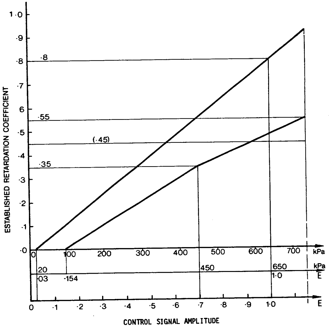
Fig. 1 SERVICE BRAKE EFFECTIVENESS REQUIREMENT (AXLE GROUPS LADEN TO GGALR)
