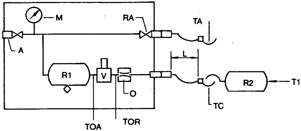
Fig. 2 CALIBRATION OF TEST RIG
