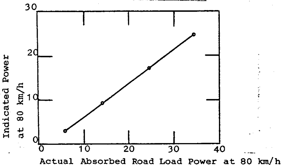
EXAMPLE OF A DYNAMOMETER CALIBRATION CURVE
