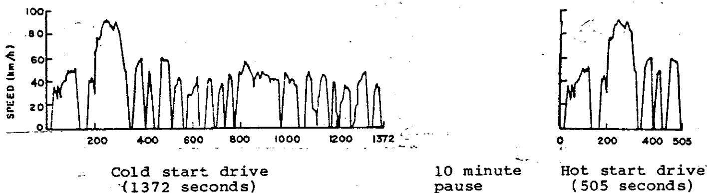
CVS-CH DRIVING SCHEDULE FIGURE I.1
