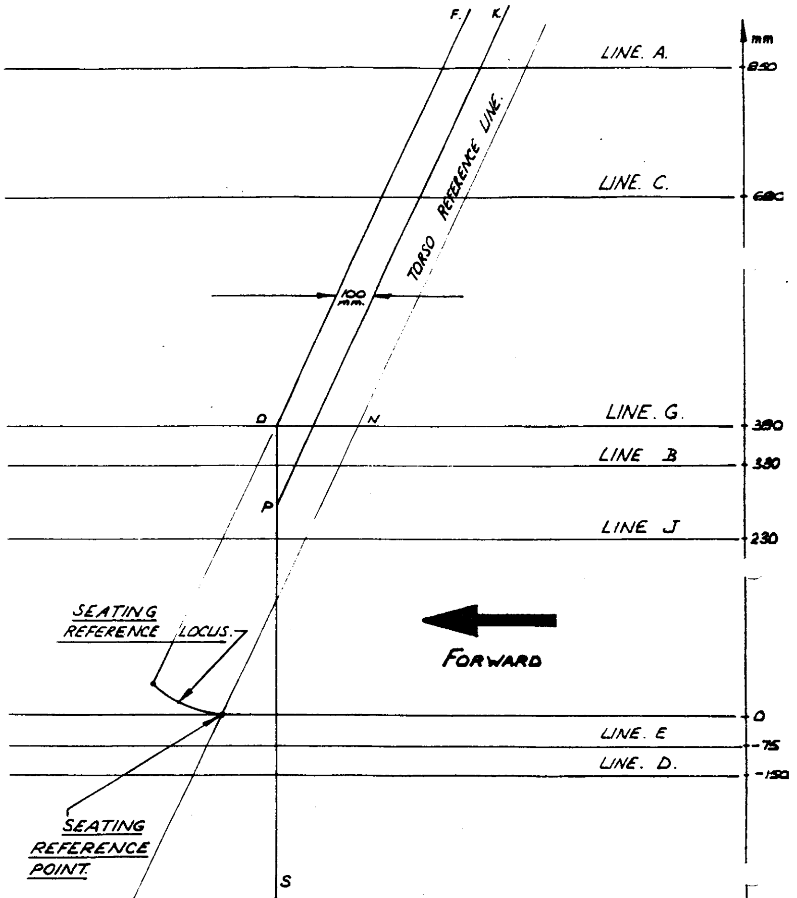
FIG. 2 COMPONENT BOUNDARY LOCATION
