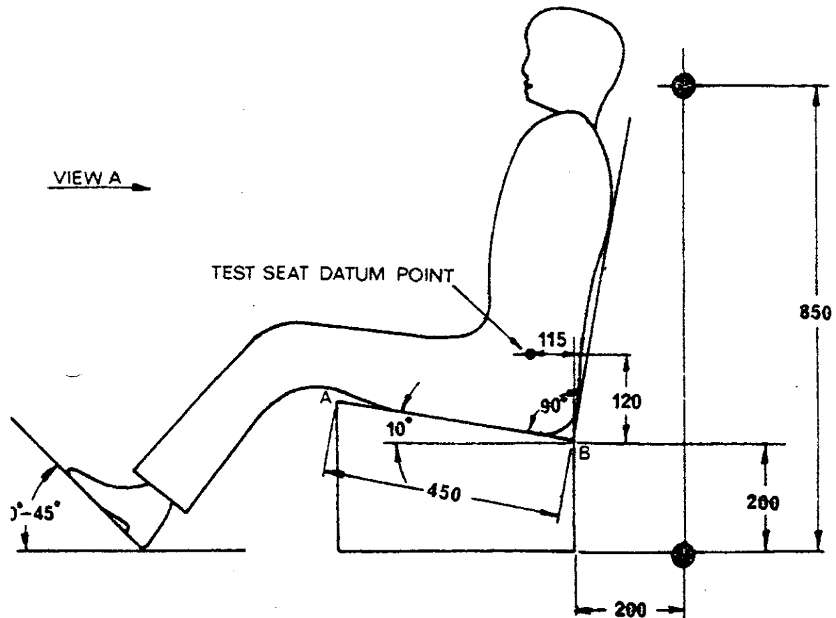
FIG. 1 TEST SEAT & ANCHORAGES
