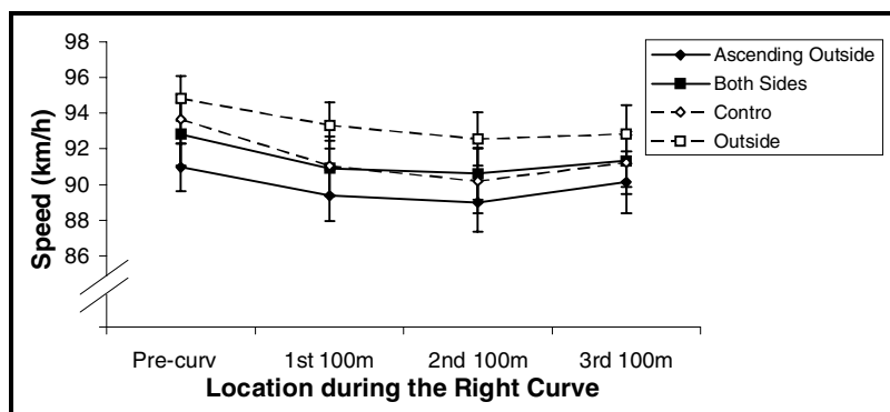
Figure 5.6: Speed ( \pm SE) on the right (outside) curve with reflector posts
