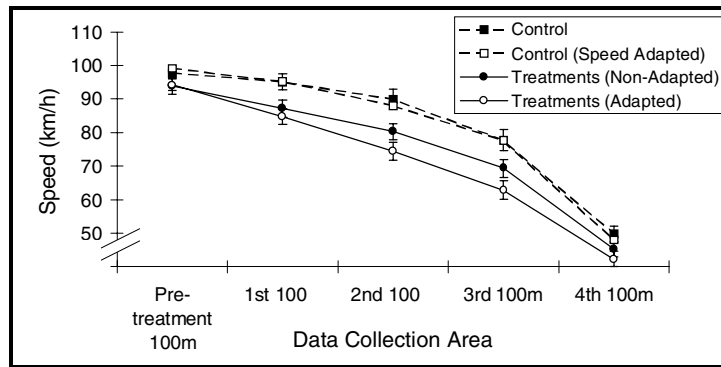
Figure 3.2: Mean speed ( \pm SE) for the control and three treatment roads (decreasing transverse lines, constant transverse lines, and peripheral transverse lines) both before and after speed adaptation.
