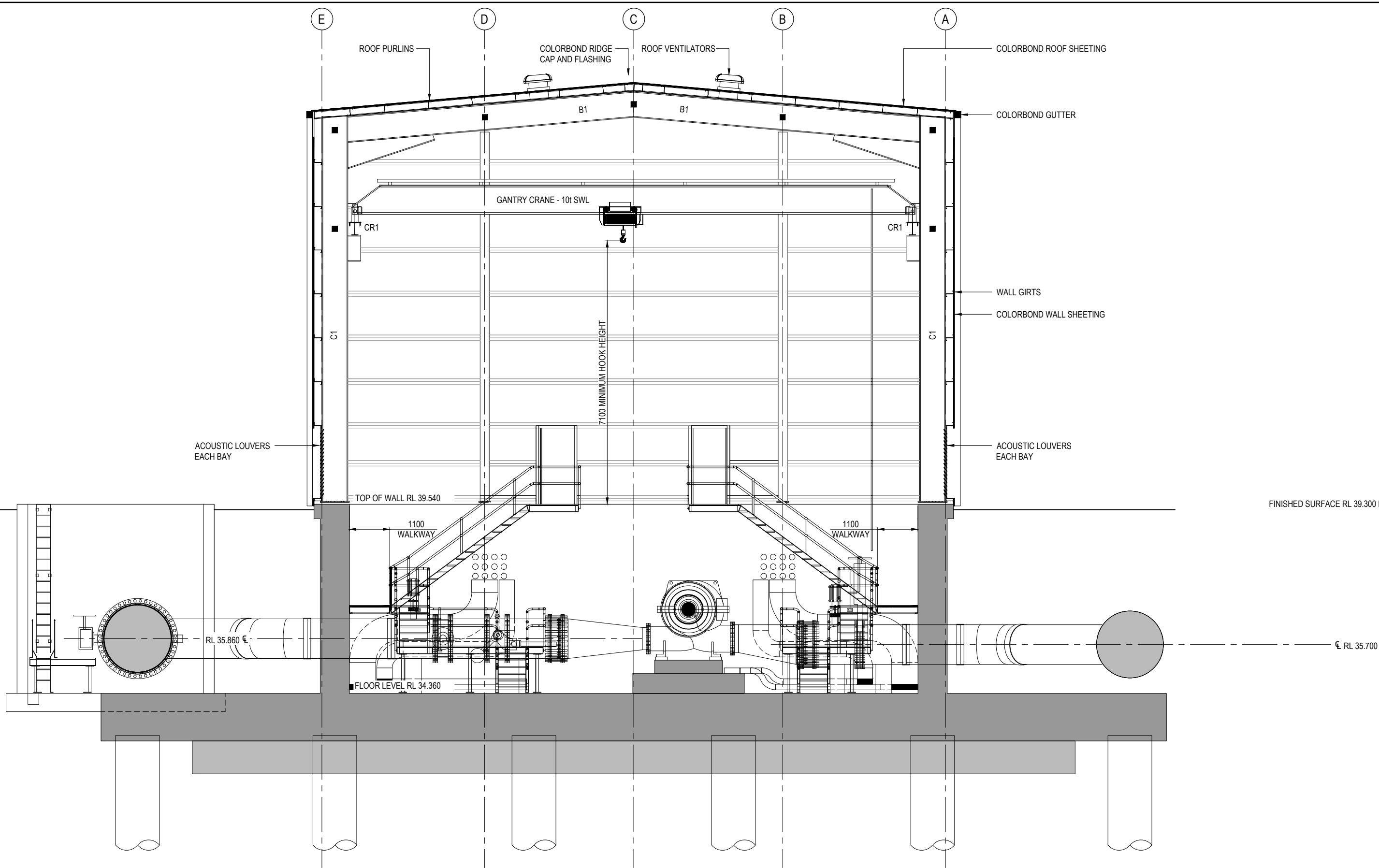
SECTION B SCALE 1:50 (A1)
