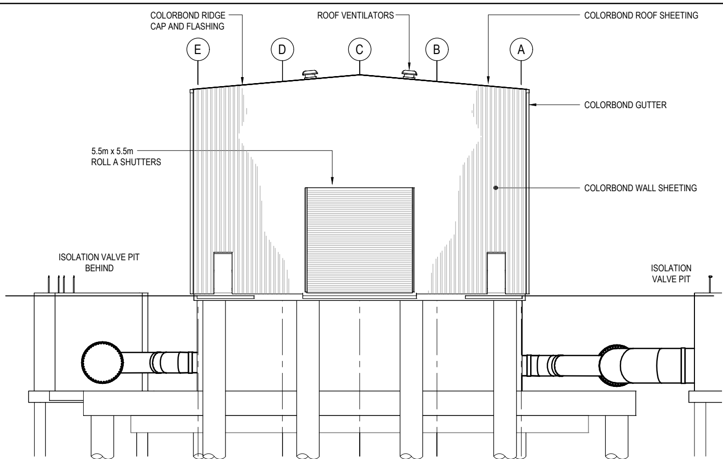
EASTERN ELEVATION SCALE 1:100
