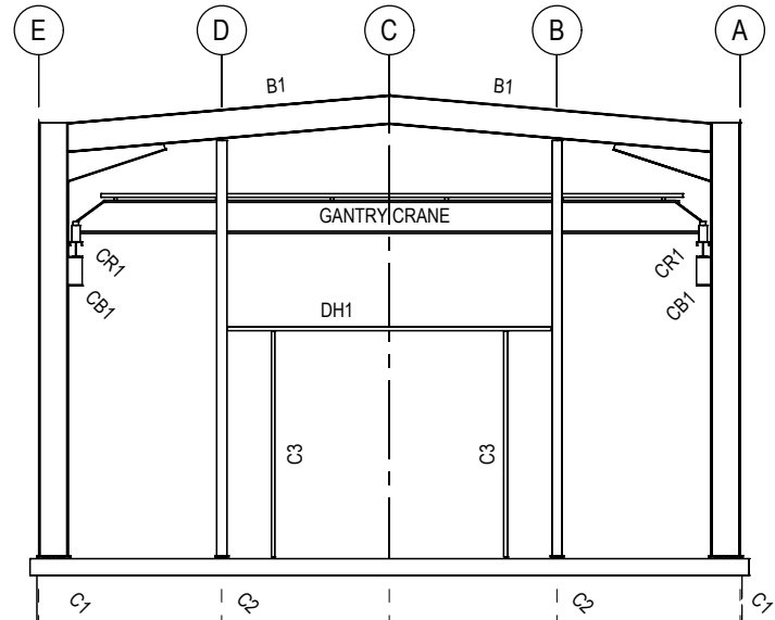
END ELEVATION - STEEL MARKING SCALE 1:100
