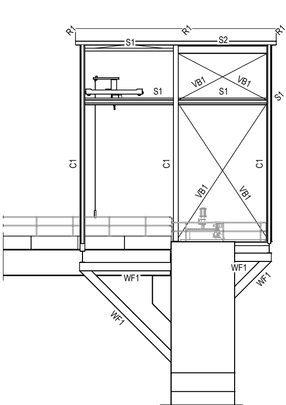
ELEVATION - STEEL MARKING SCALE 1:100
