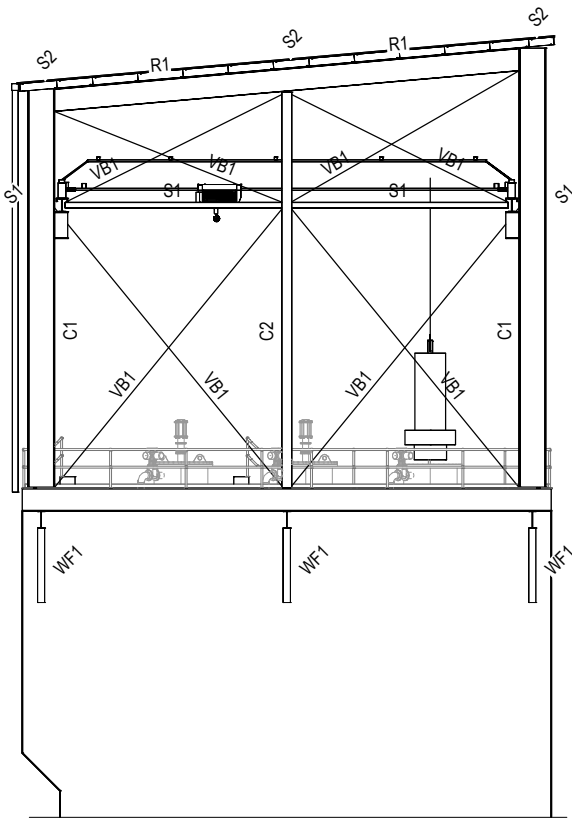
END ELEVATION - STEEL MARKING SCALE 1:100
