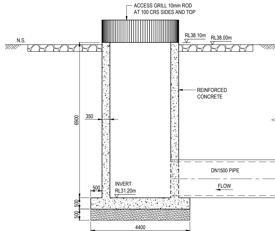
SECTION A SCALE 1:50
