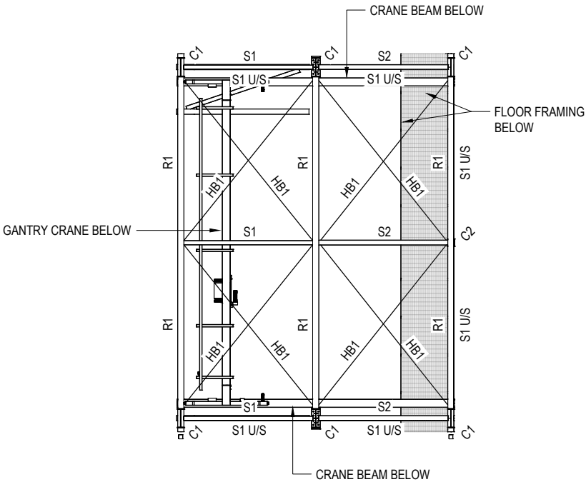
PLAN - STEEL MARKING SCALE 1:100
