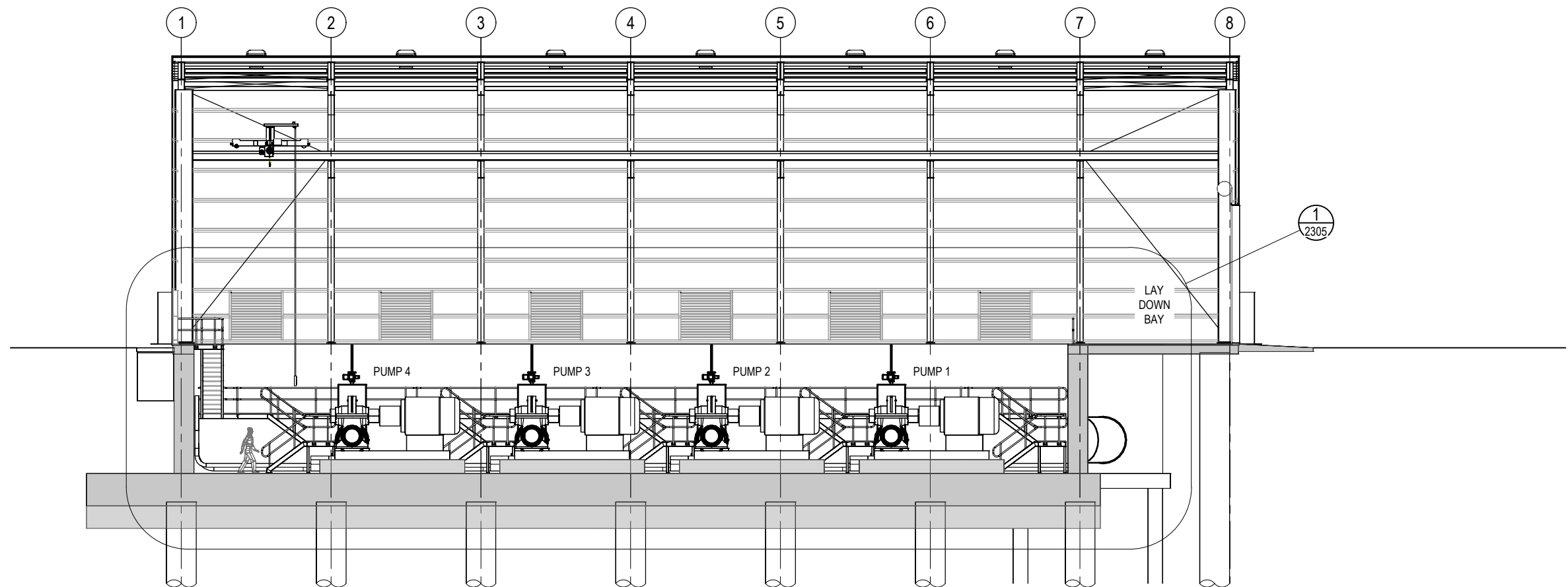
SECTION A-A SCALE 1:100 (A1) 2300
