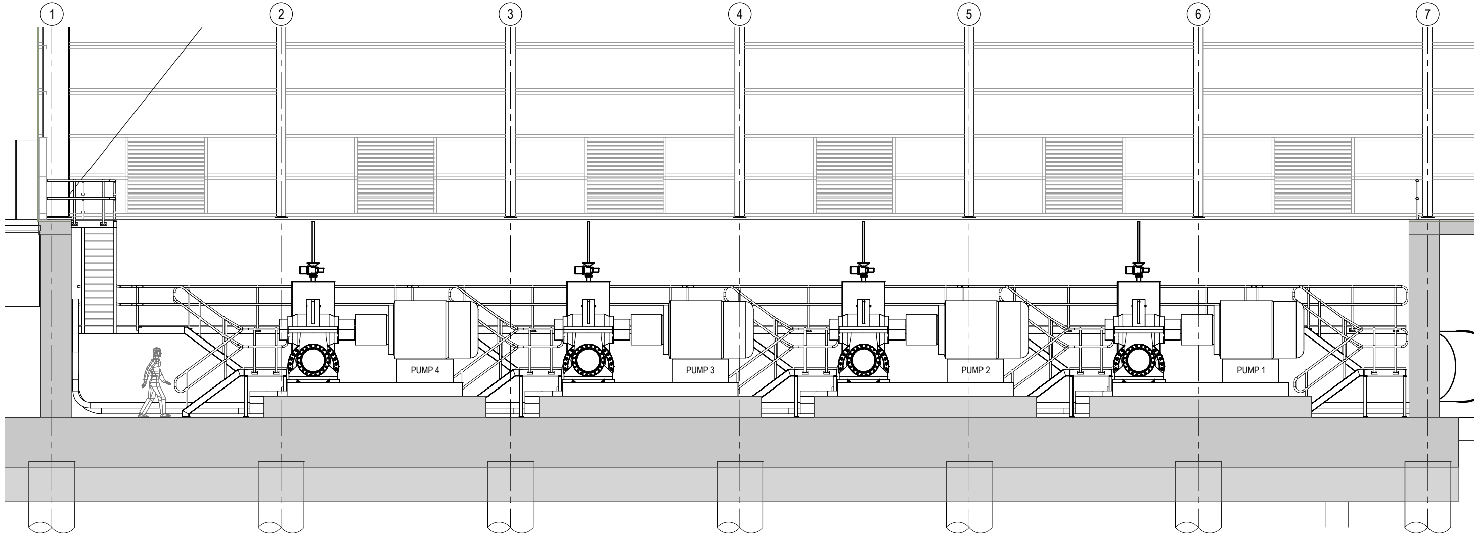
DETAIL SCALE 1:50 (A1) 1/2302
