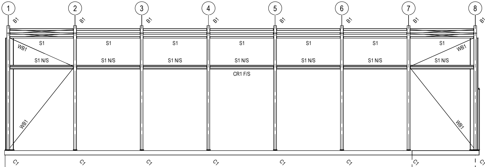
ELEVATION - STEEL MARKING SCALE 1:100
