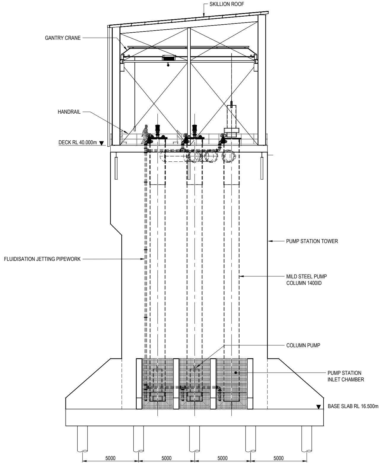
ELEVATION SCALE 1:100
