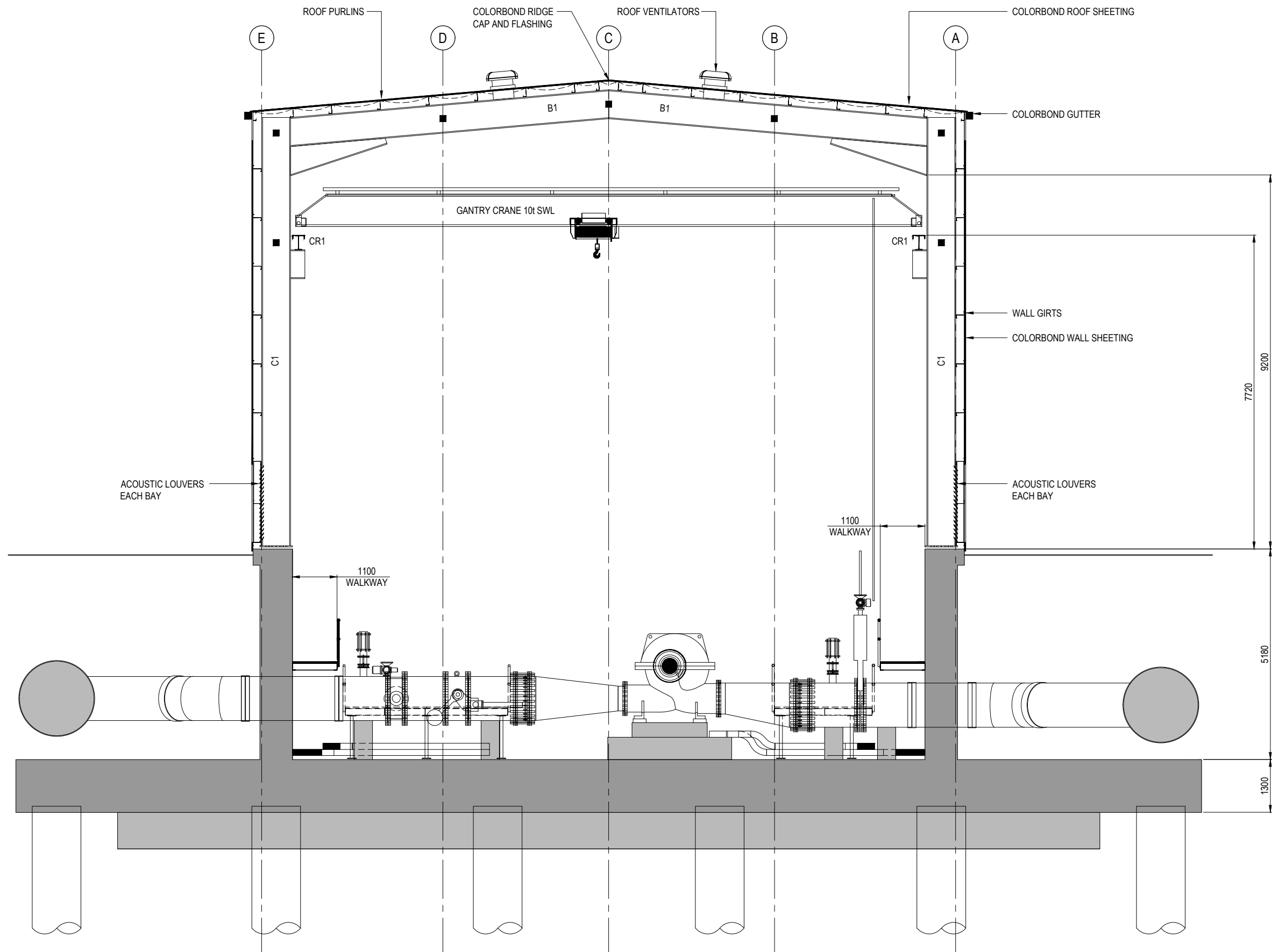
TYPICAL SECTION SCALE 1:50 (A1)
