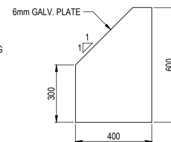
TYPICAL FLOW VANE DETAIL SCALE 1:10
