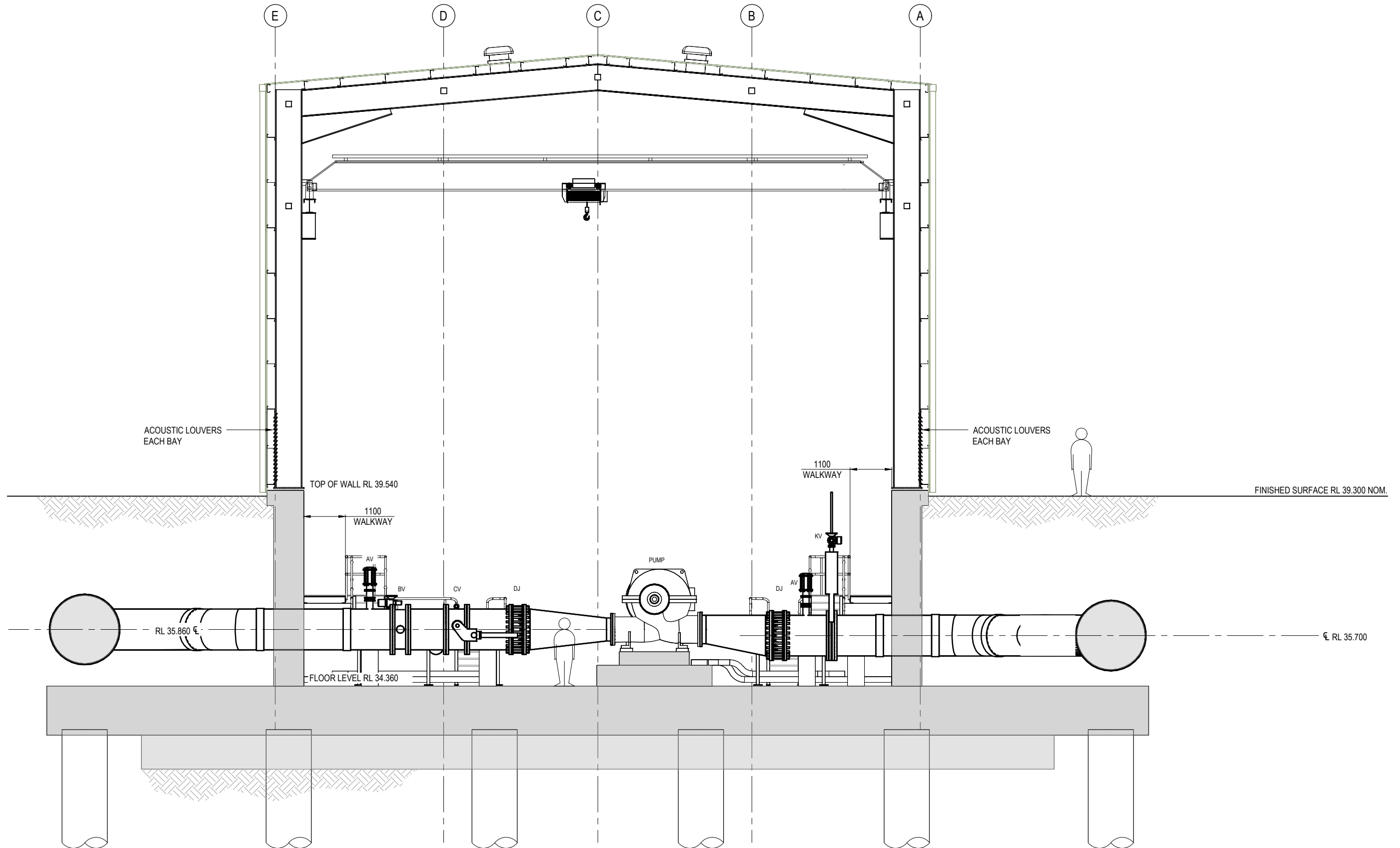
SECTION C SCALE 1:50 (A1) 2300
