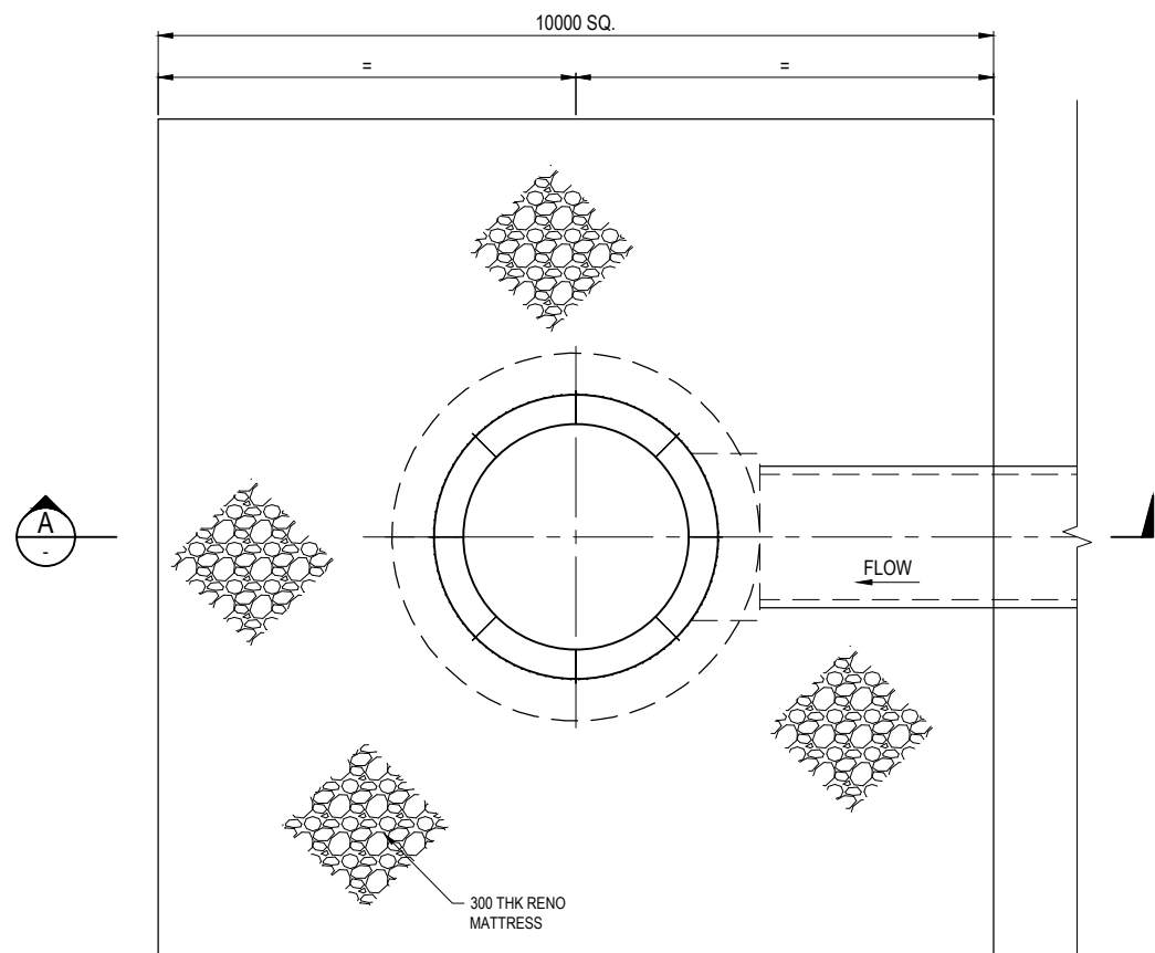
OVERFLOW OUTLET STRUCTURE SCALE 1:50
