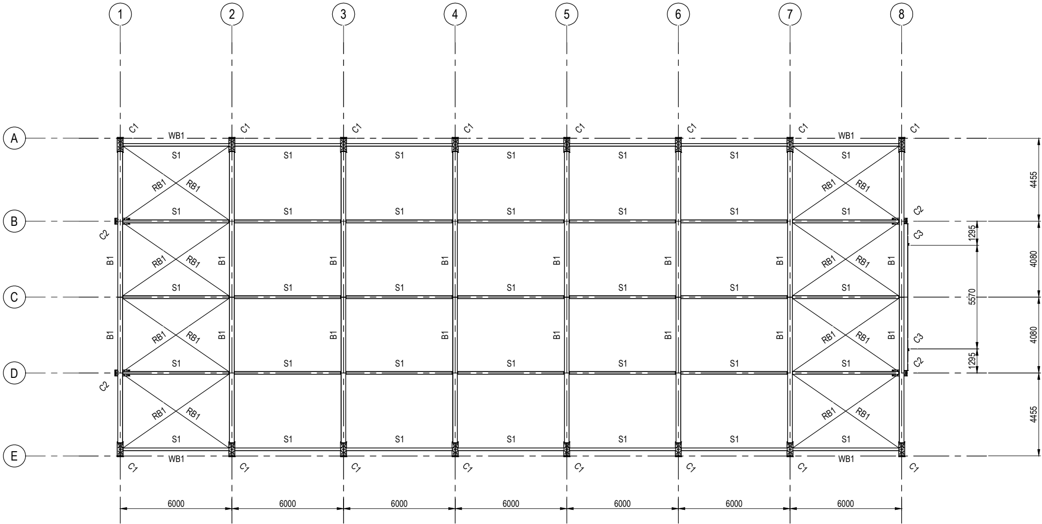
PLAN - STEEL MARKING SCALE 1:100
