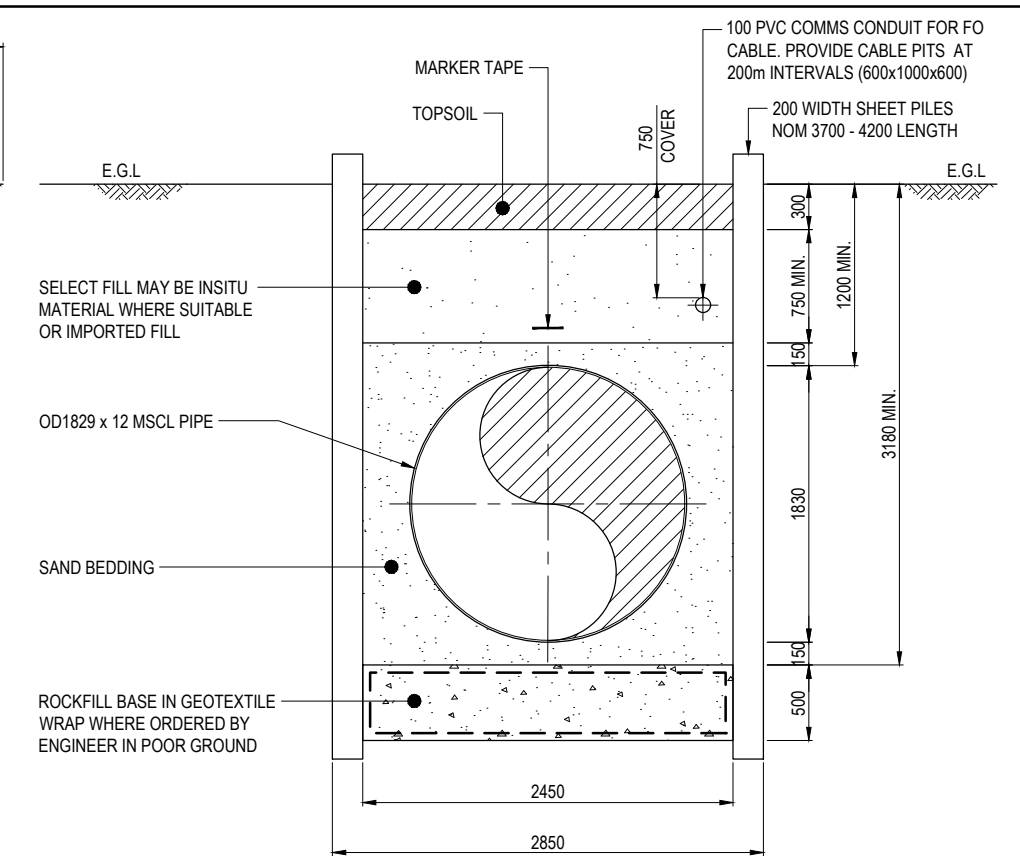
TRENCH TYPE B - SHEET PILED EXCAVATION SCALE 1:25
