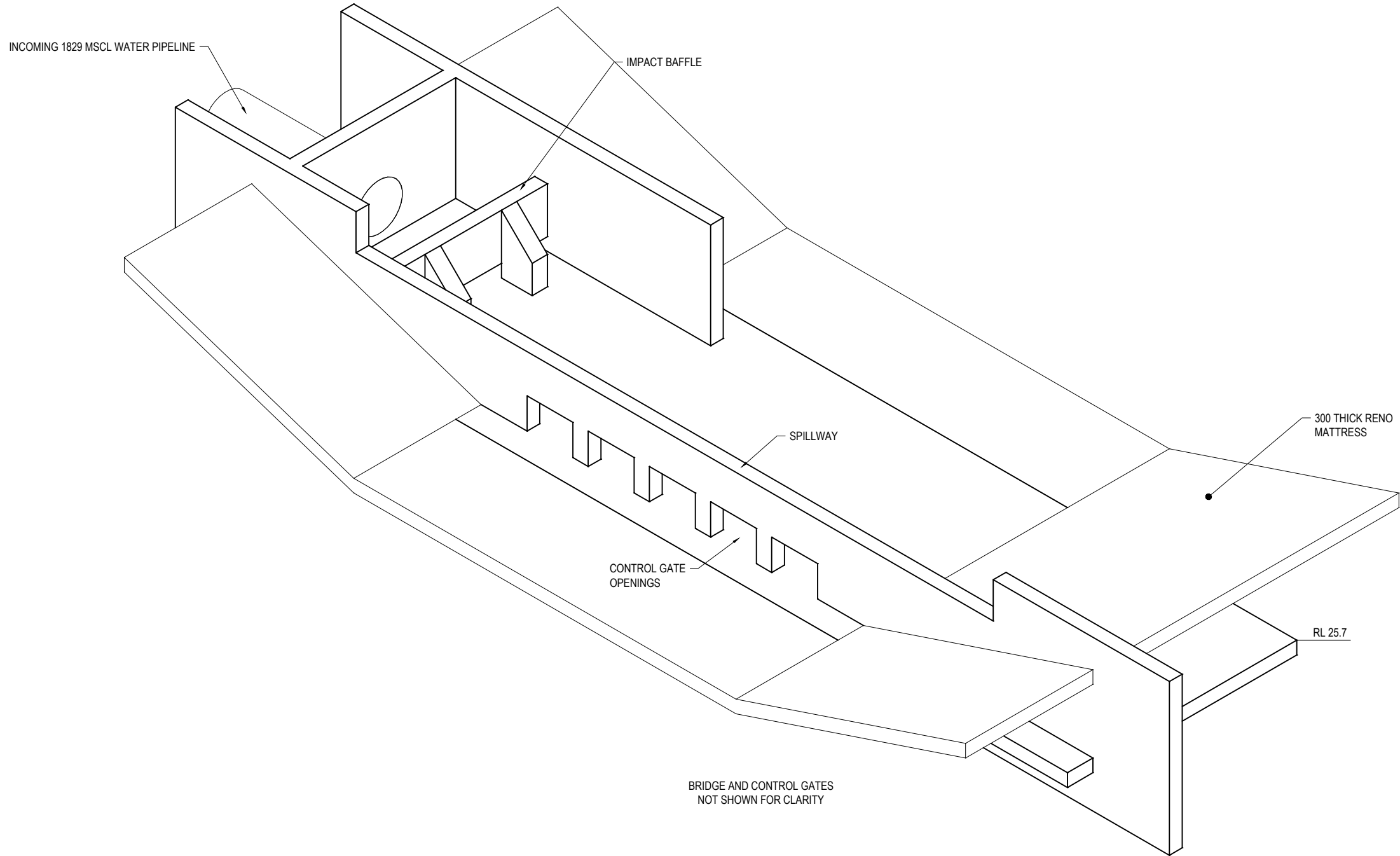
PICTORIAL NTS
