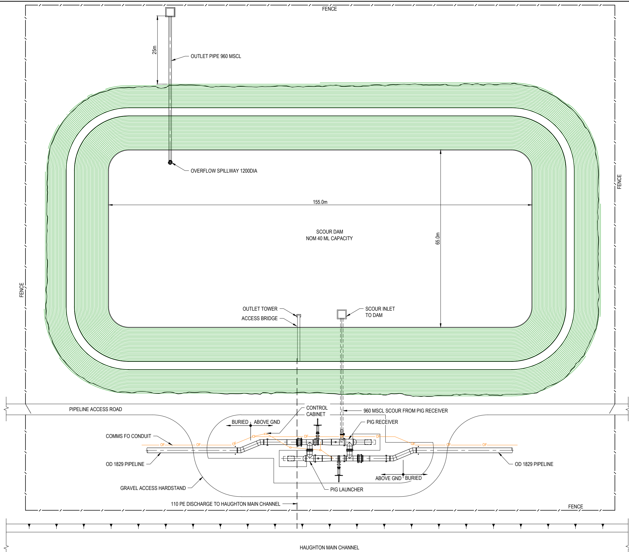
PLAN SCALE 1:400 (A1)
