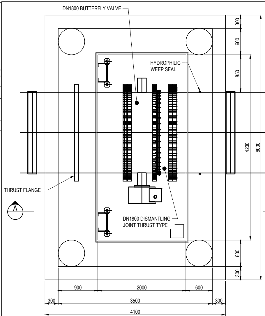
PLAN SCALE 1:25
