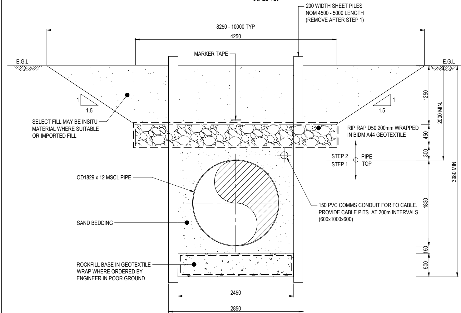
TRENCH TYPE C - MAJOR WATERWAY CROSSING SCALE 1:25
