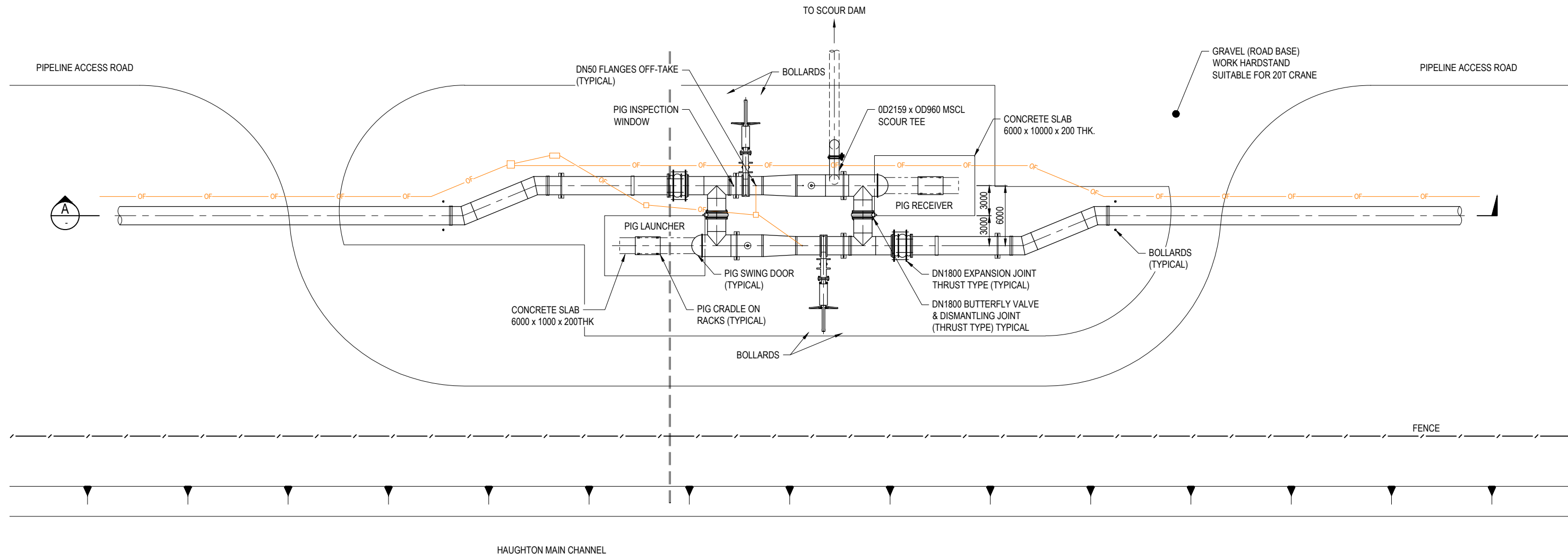
PLAN SCALE 1:200 (A1)
