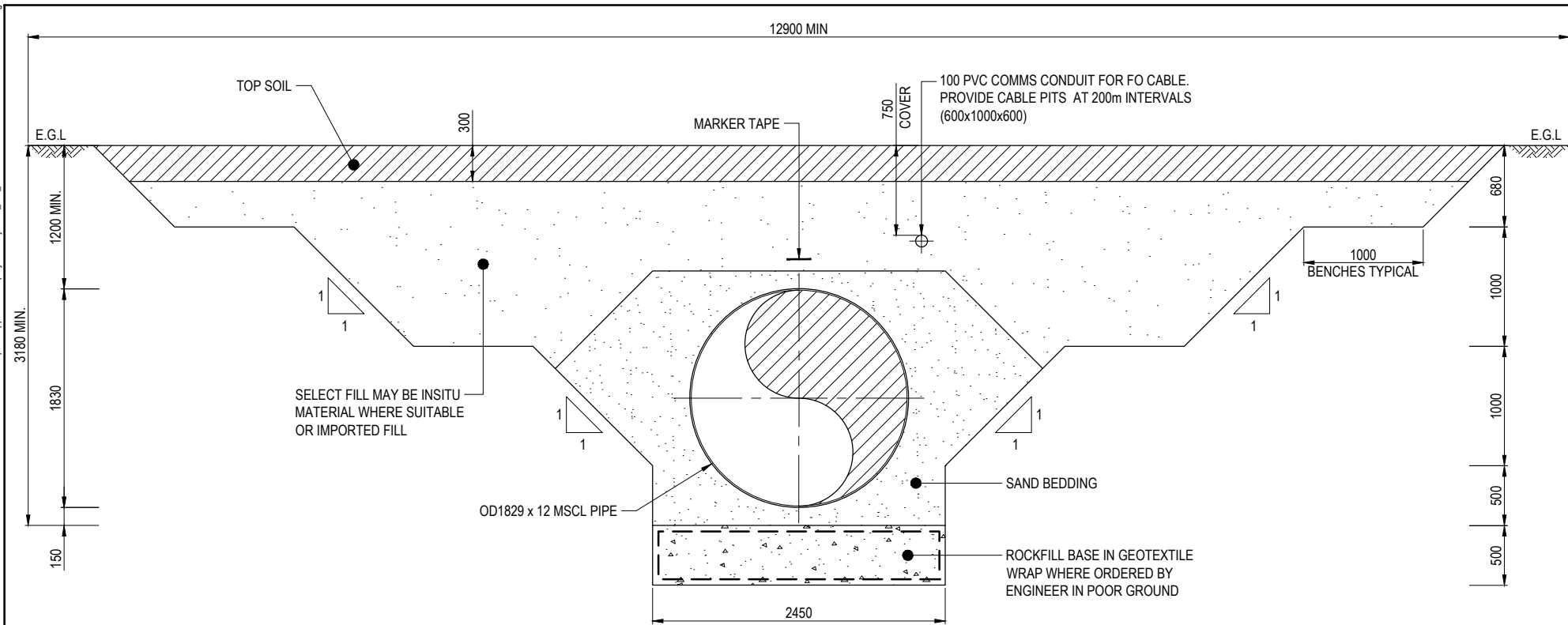
TRENCH TYPE A - OPEN EXCAVATION SCALE 1:25
