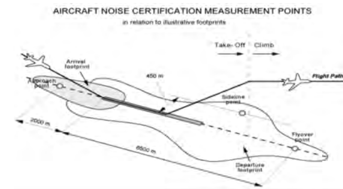
Figure 3 Certification Measurement Points 8 8 Reproduced from ERCD Report 0205 Quota Count Validation Study: Noise Measurements and Analysis, Civil Aviation Authority
