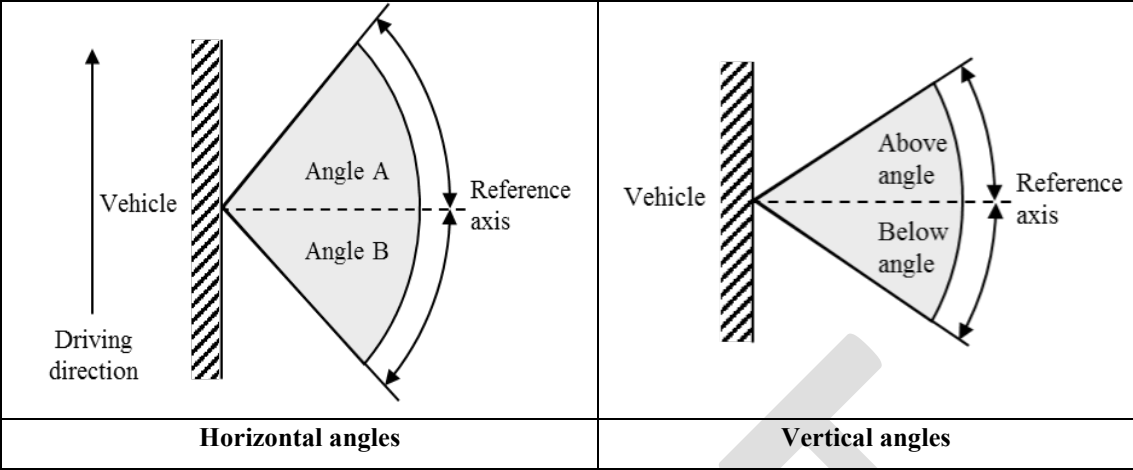
Figures A2-III Angles of geometric visibility, horizontal and vertical
