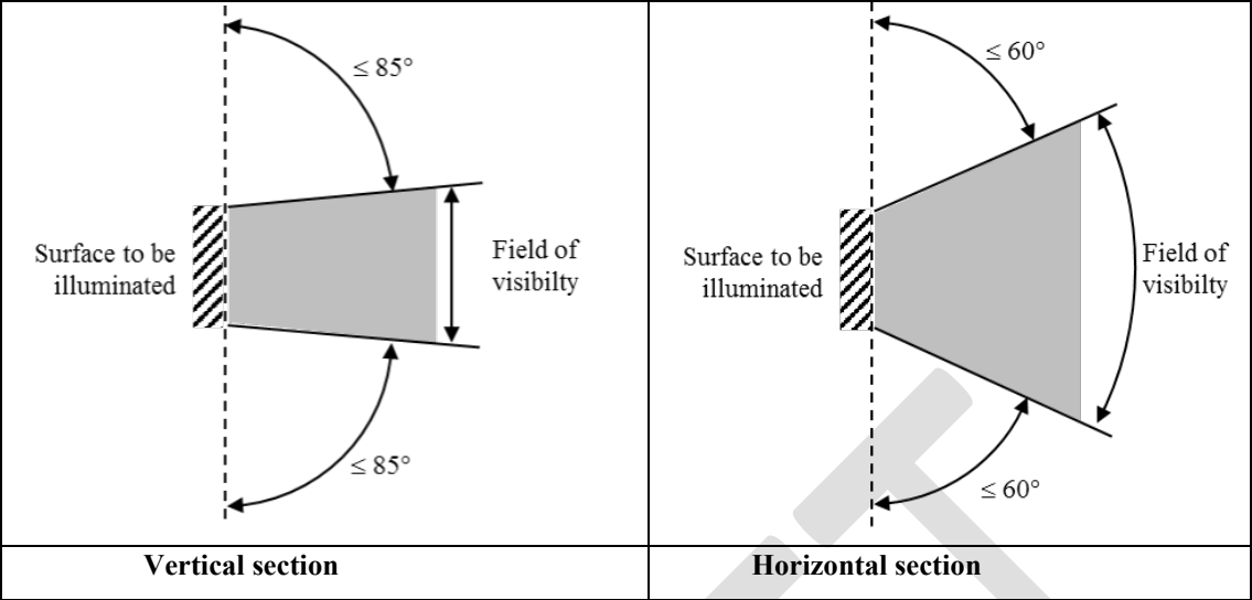
Figures A2-IV Field of visibility, horizontal and vertical
