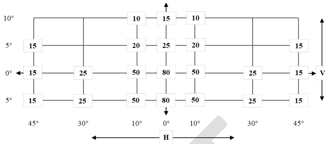
Figure A3-V Light distribution for reversing lamps
